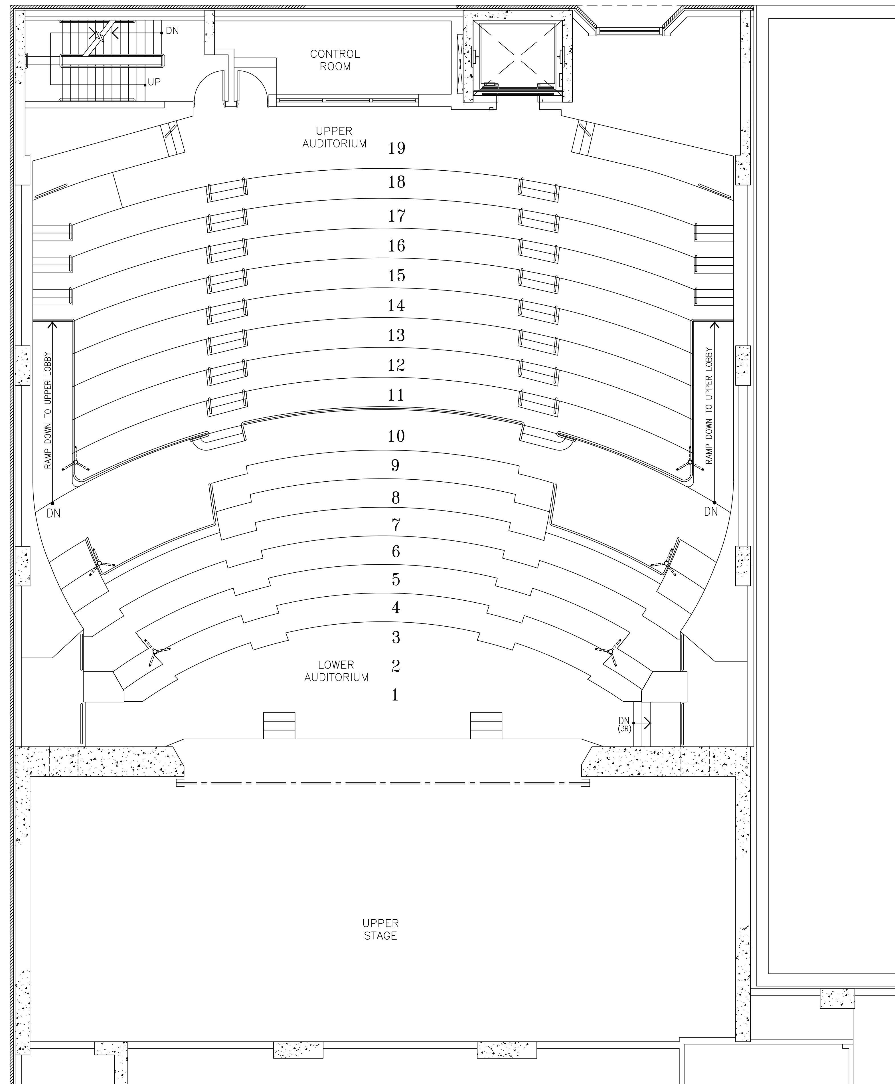
AUDITORIUM PLAN
